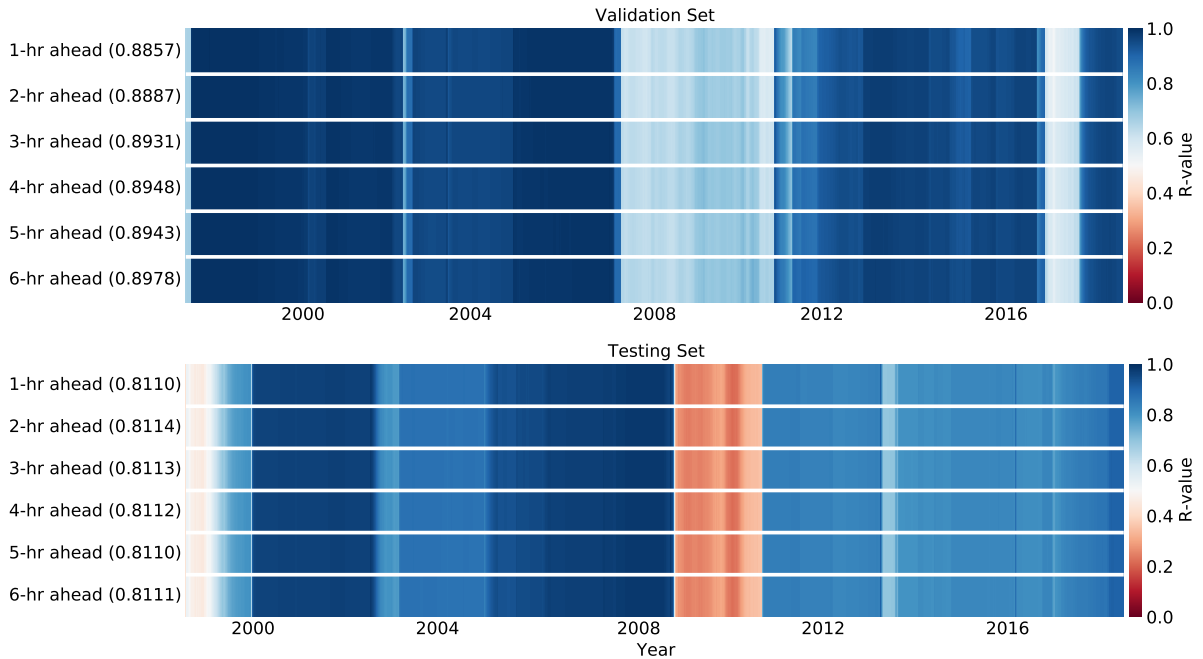
Figure 4.13: Temporal heatmap shows a comparison between the model outputs and observations for the rolling-mean window correlation of the integral >10 MeV proton flux at six predicting windows. The top panel represents the validation set and the bottom panel represents the testing set. The numbers on the y-axis are the mean R values.
