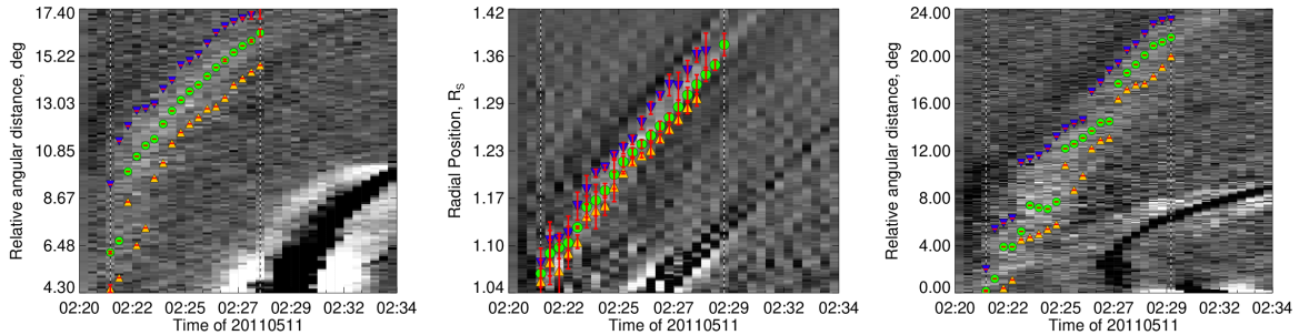
Figure 2.3: J-map plots for the event of May 11, 2011, for the radial direction (middle plot) and the left and right flanks of the wave in the lateral heliocentric direction (the left and right plots, respectively). Blue, green, and orange filled symbols are the positions of the CBF front, peak, and back, respectively. The uncertainty of the average measurements is shown as red bars.
