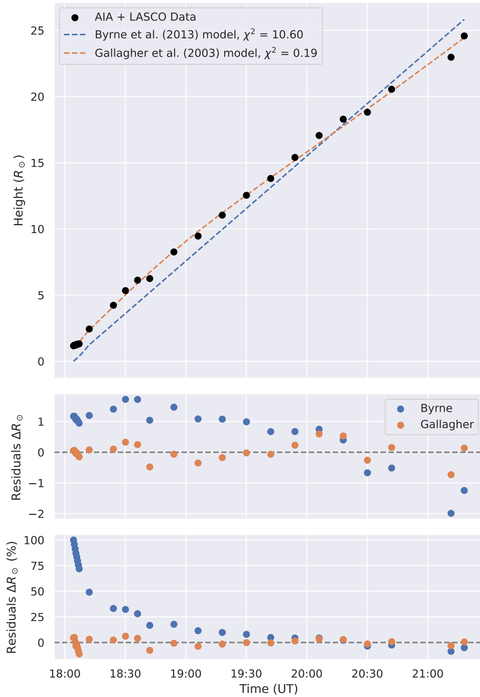
Figure A.7: Same for the event on August 8, 2011.
