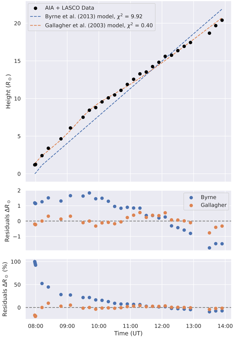
Figure A.16: Same for the event on October 25, 2013.
