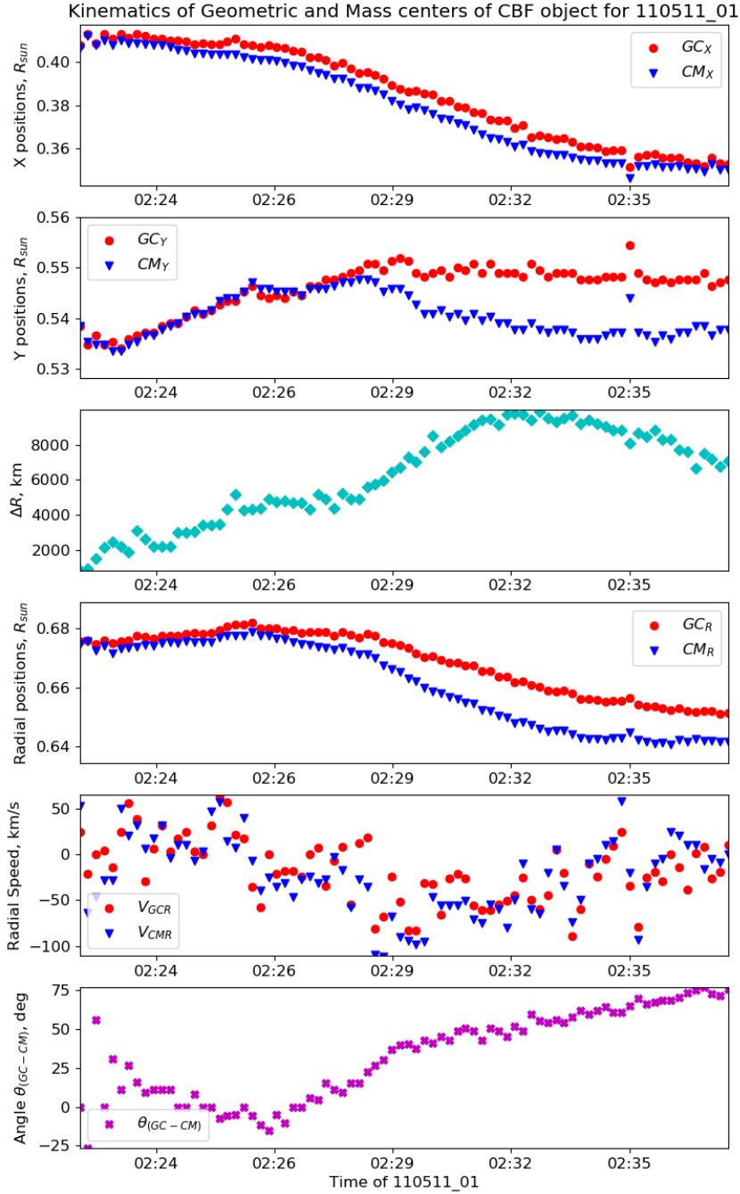
Figure 2.17: Analysis of the center of mass and geometric centers' motion during the May 11, 2011 event. The different rows present the X-, Y-, and R- positions for both GC and CM, the distance between GC and CM in km , and the angle between these two points over time. Credit goes to Stepanyuk et al. (2022).
