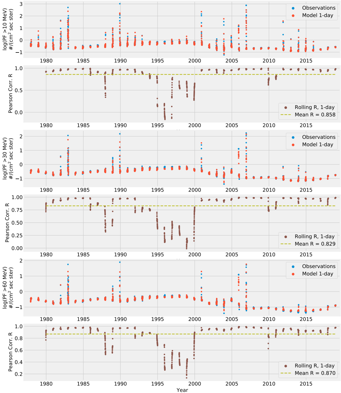
Figure 4.9: Comparison between the model outputs and observations of the test set for the 3 energy channels. In addition to the rolling-mean window correlation for 1-day ahead predictions.
