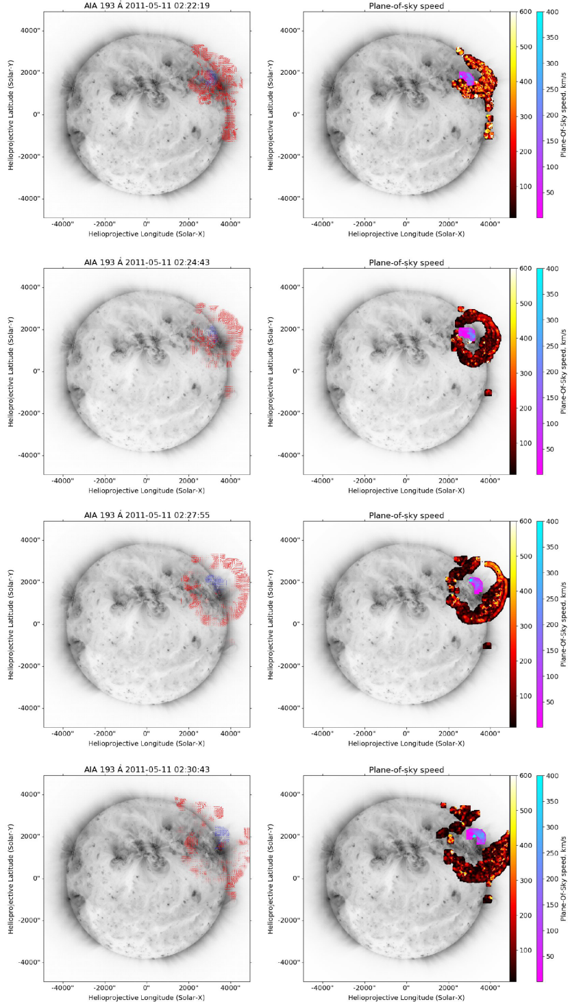
Figure 2.16: FLCT model output for four image pairs from Fig. 3. Left: the plane-of-sky velocity vectors. Right: plane-of-sky speed. Credit goes to Stepanyuk et al. (2022).
