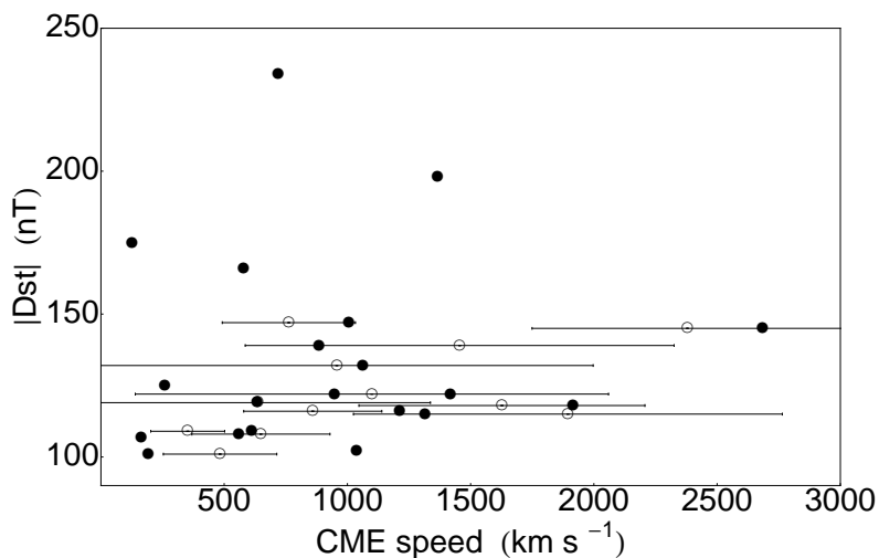
Figure 2.20: Scatter plot illustrating the relationship between the Dst index and CME speed, incorporating data from the SOHO/LASCO instrument (represented by filled circles) and 3D de-projections (depicted by empty circles). Credit goes to Miteva et al. (2023).
