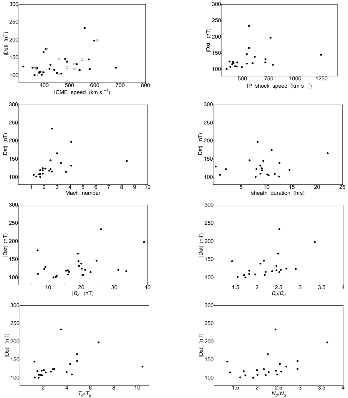
Figure 2.21: Comprehensive scatter plots illustrating the relationships between Dst index and various solar wind parameters, including Wind/ACE ICME speed, IP shock speed, Mach number, duration of sheath region, B_z , magnetic field jump, temperature jump, and density jump. Credit goes to Miteva et al. (2023).
