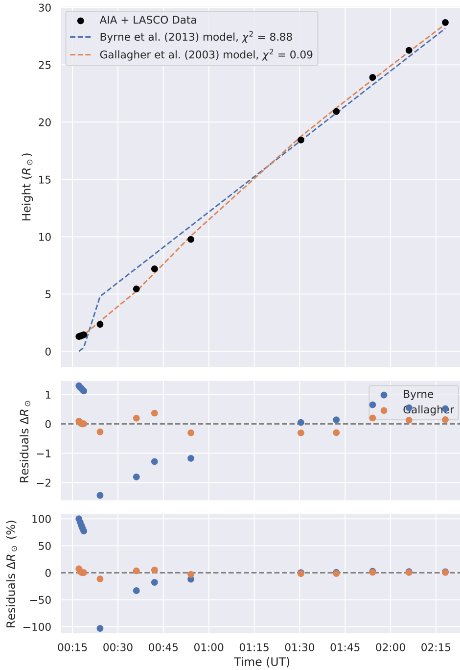
Figure A.8: Same for the event on March 7, 2012.
