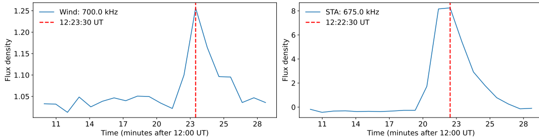
Figure A.27: Cut of the flux density at 700 kHz observed by Wind (left panel) and STEREO-A (right panel). Note: for STEREO-A, there is no exact frequency channel at 700 kHz; therefore we selected the nearest one (675 kHz).
