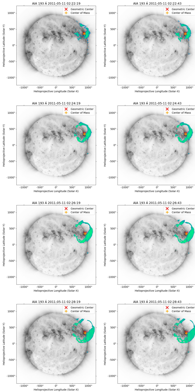
Figure 2.15: Wavetrack images of a May 11, 2011 eruption, with CBF mask applied. Four image pairs shown, separated by 2 minutes, to track CBF over time. Credit goes to Stepanyuk et al. (2022).
