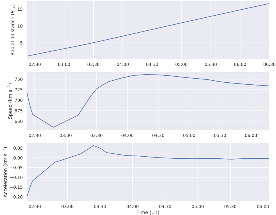
Figure 2.8: Extrapolated radial kinematics for the event occurred on May 11, 2011, based on the ballistic model of Gallagher et al. (2003) up to 17 R_{\odot} .
