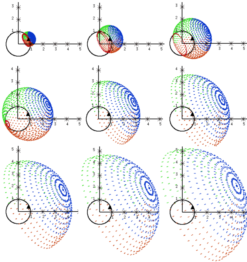
Figure 2.4: Synthetic shock model divided into three segments; the cap zone in blue and the flank zones are in red and green.
