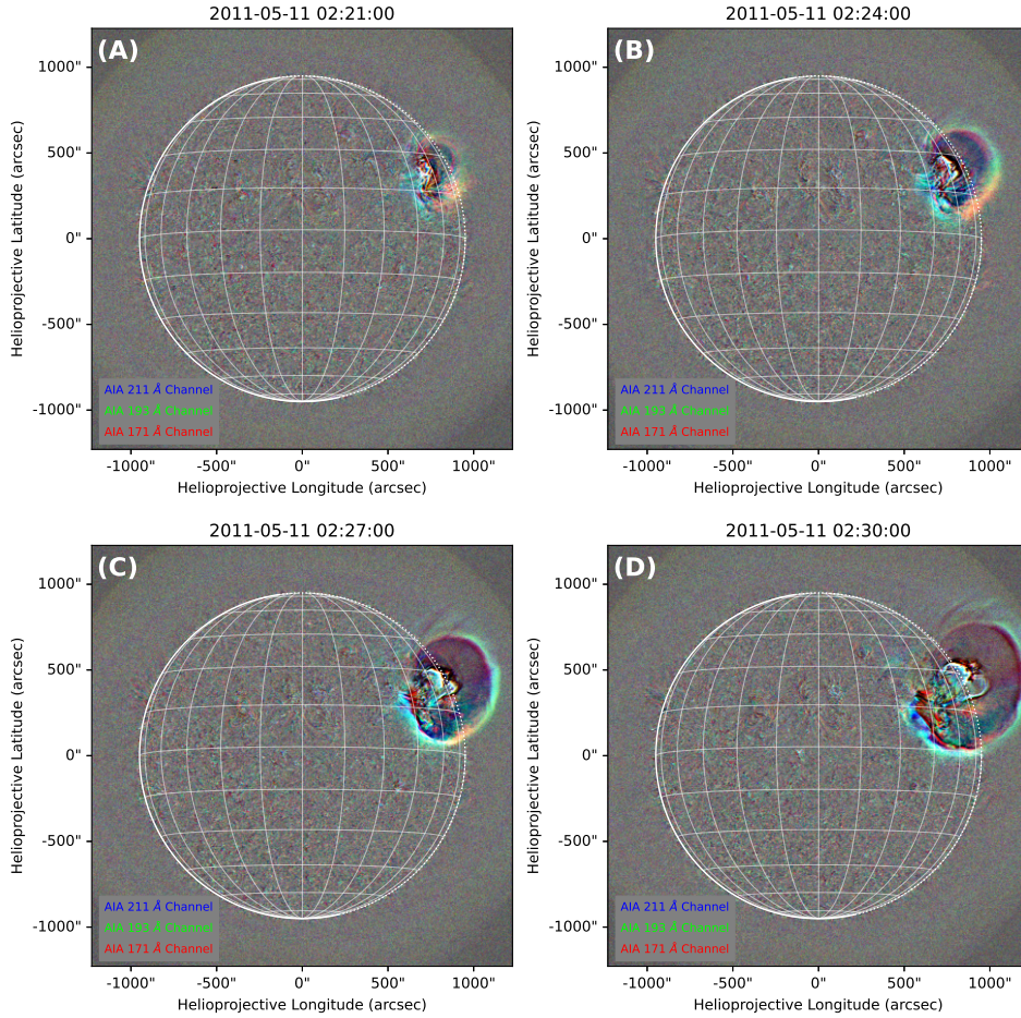
Figure 2.5: AIA running-difference images capture a coronal wave evolving over 9 minutes near the Sun's western limb, exhibiting markedly changing intensity and structure as observed in 171, 193, and 211 \text{\AA} .
