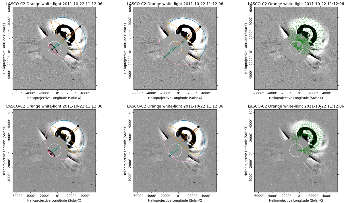
Figure 2.18: 3D reconstructions of a CME (E03) using the spheroid, ellipsoid, and GCS model from the PyThea tool performed by observers 1 and 2 (top and bottom row, respectively). Credit goes to Miteva et al. (2023).
