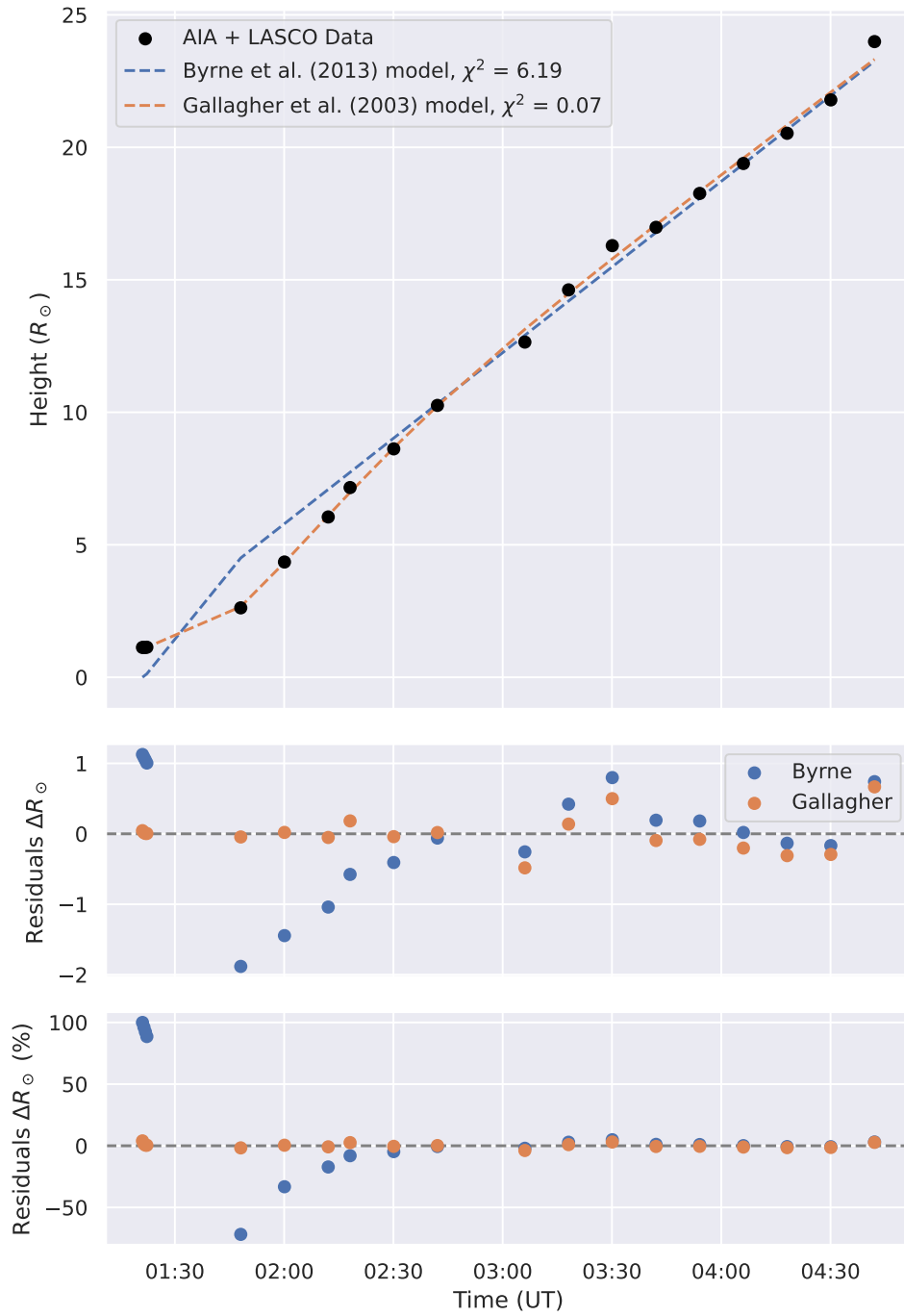
Figure A.13: Same for the event on May 15, 2013.
