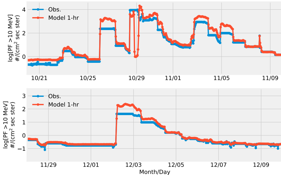
Figure 4.16: Comparison between the model's forecast and the observations for the integral >10 MeV proton flux at forecast horizon of 1 hour ahead. The top panel represents a sample of the validation set and the bottom panel represents a sample of the testing set.
