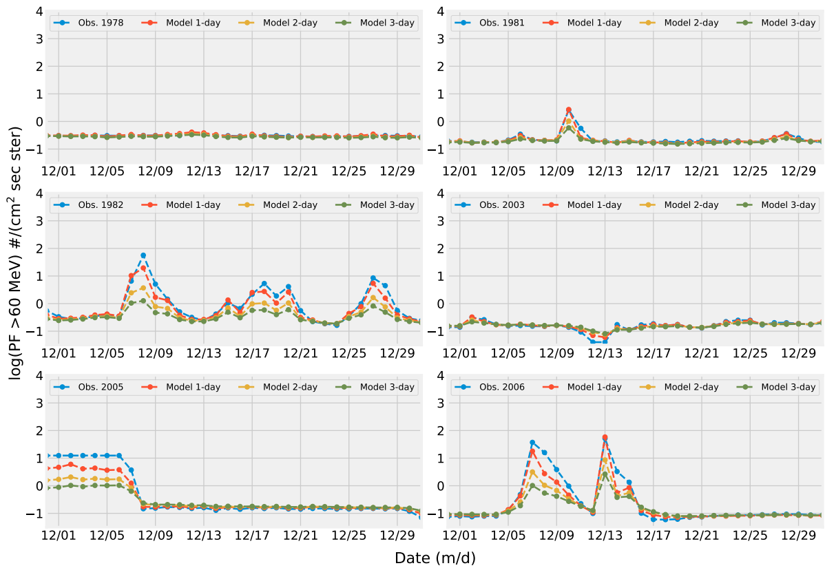
Figure 4.12: The model's forecasts for the out-of-sample testing set for the >60 MeV channel are shown at forecast horizons of 1 day, 2 days, and 3 days ahead, using samples of data from December in selected years mentioned in the top-left side of the plots.
