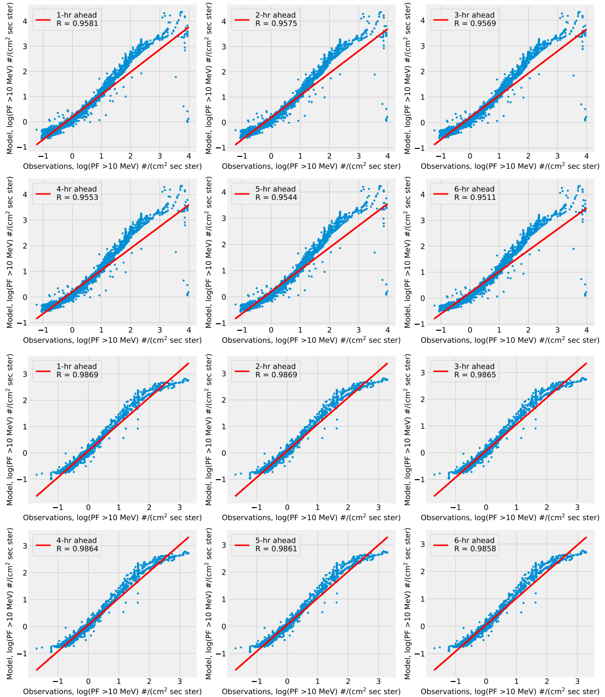
Figure 4.14: Correlation between model predictions and observations for the integral >10 MeV proton flux of the validation (top two rows) and testing (bottom two rows) sets.
