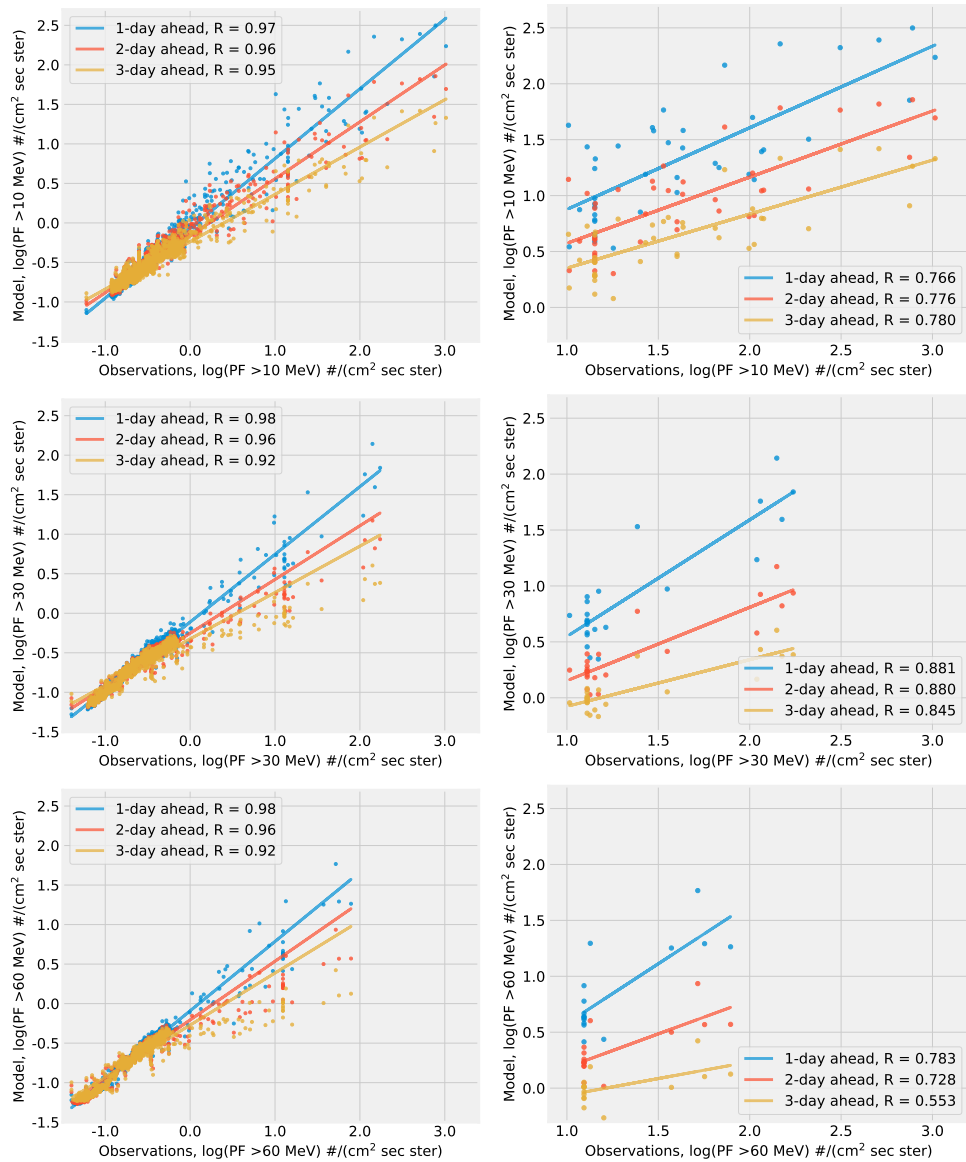
Figure 4.8: Same as Figure 4.7 but for the test set.
