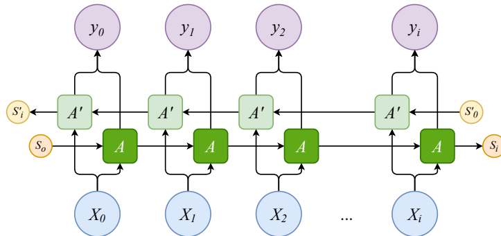
Figure 4.3: Architecture of a single BiLSTM layer. The blue circles at the bottom labeled by (x_0, x_1, x_2, \dots, x_i) are the input data values at multiple time steps. The purple circles, on the other hand, are the output data values at multiple time steps labeled by (y_0, y_1, y_2, \dots, y_i) . The dark green and light green boxes are the activation units of the forward layer and the backward layer, respectively. The orange and yellow circles are the hidden states at the forward layer and the backward layer, respectively. Both the forward and backward layers compose a single hidden BiLSTM layer. The figure is adopted from Olah (2015)
