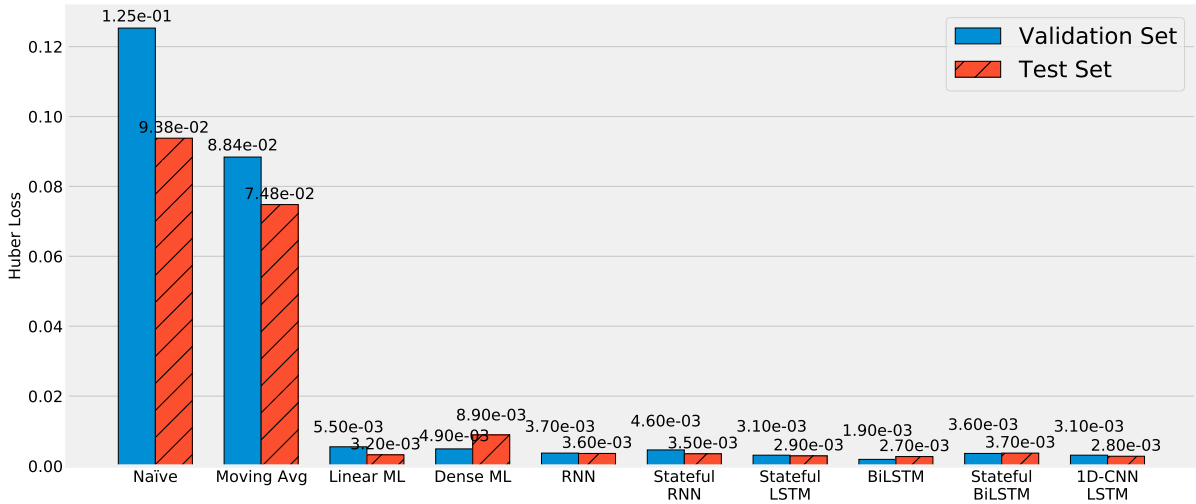
Figure 4.5: Benchmarking of 10 models, shows the Huber loss for the validation and test sets.
