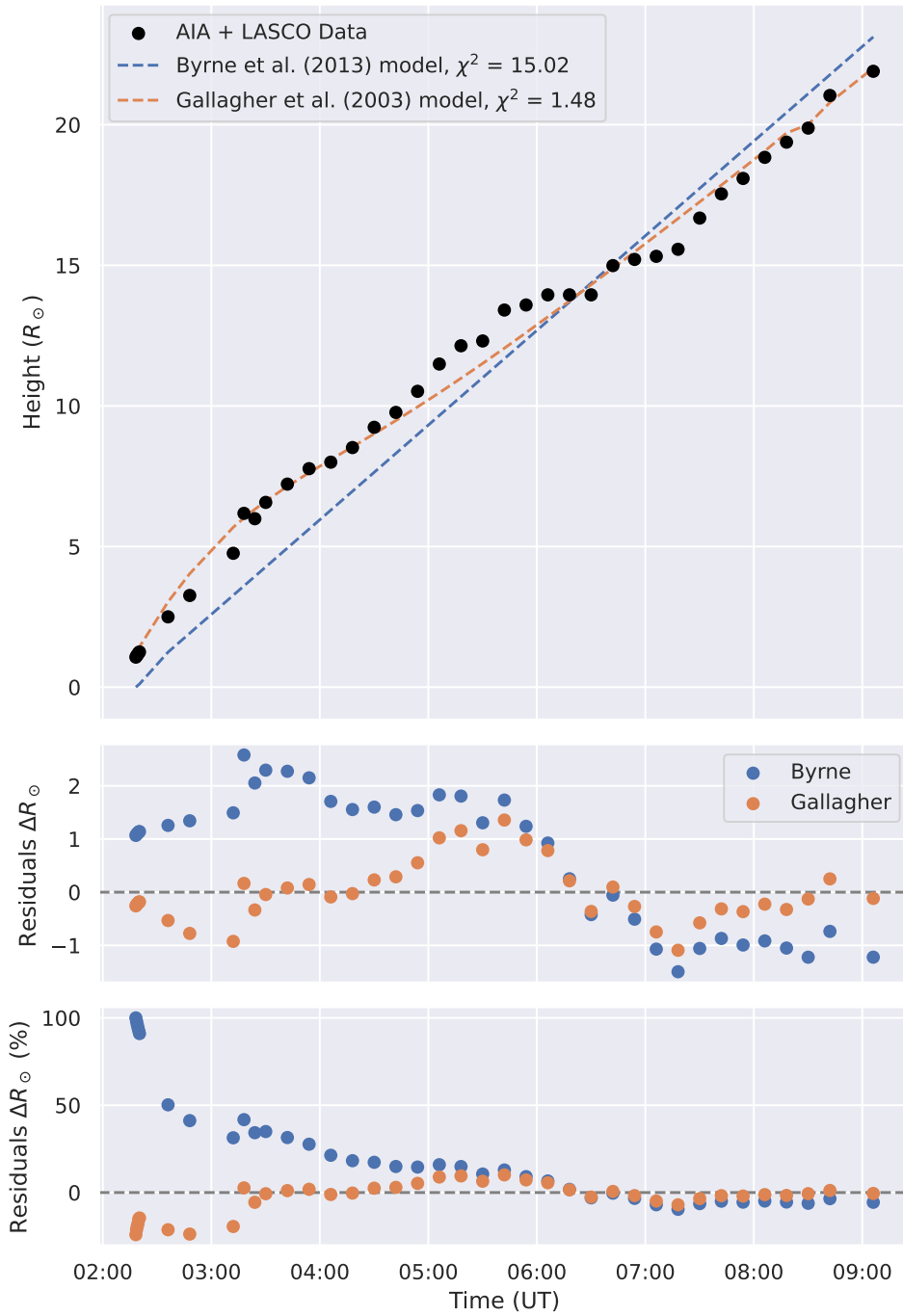
Figure A.23: Same for the event on October 29, 2015.
