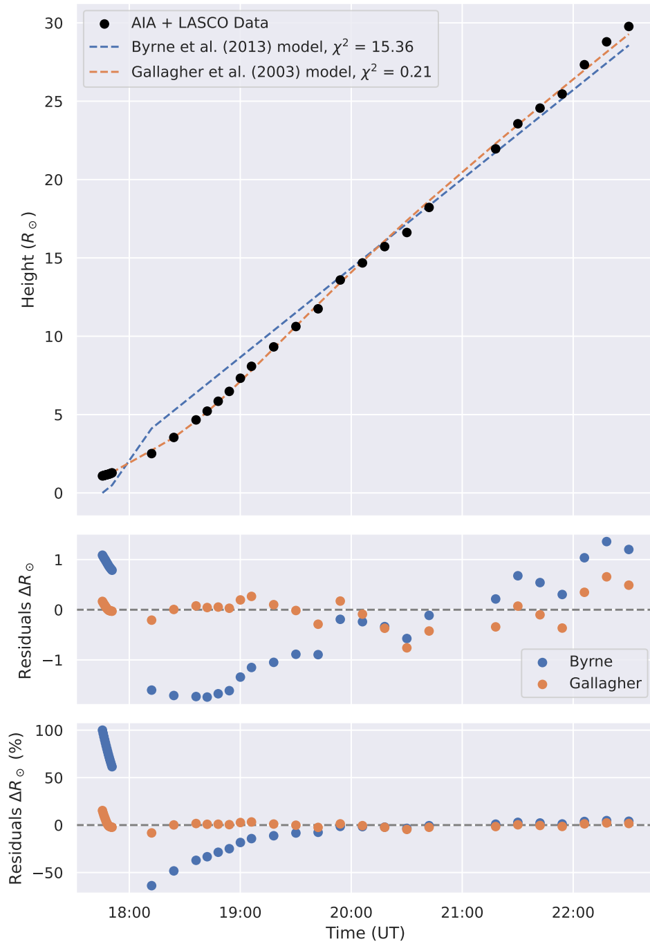
Figure A.22: Same for the event on September 20, 2015.
