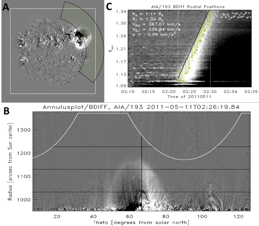
Figure 2.2: Illustration for the annulus method used to extract kinematic data from AIA images. (A) shows the full Sun disk with the relevant region highlighted for analysis (green sector). The white box outlines the AIA FOV. (B) displays the extracted annular region mapped onto polar coordinates, with the actual data extent marked by the white curve. Black lines indicate the directions used for measuring radial and lateral motions. (C) shows a stacked plot of intensity along the radial direction, with green markers highlighting intensity peaks and their corresponding distances from the CBF wavefront. The white lines represent the time interval during which the CBF is tracked within the AIA FOV. This figure is curated from (Kozarev et al. 2017).
