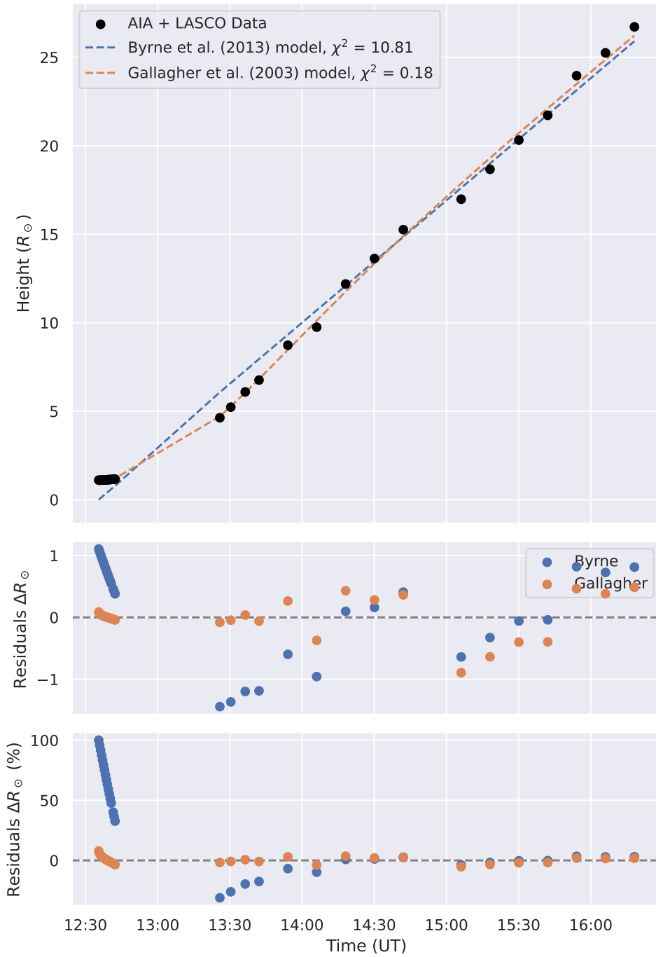
Figure A.14: Same for the event on May 22, 2013.
