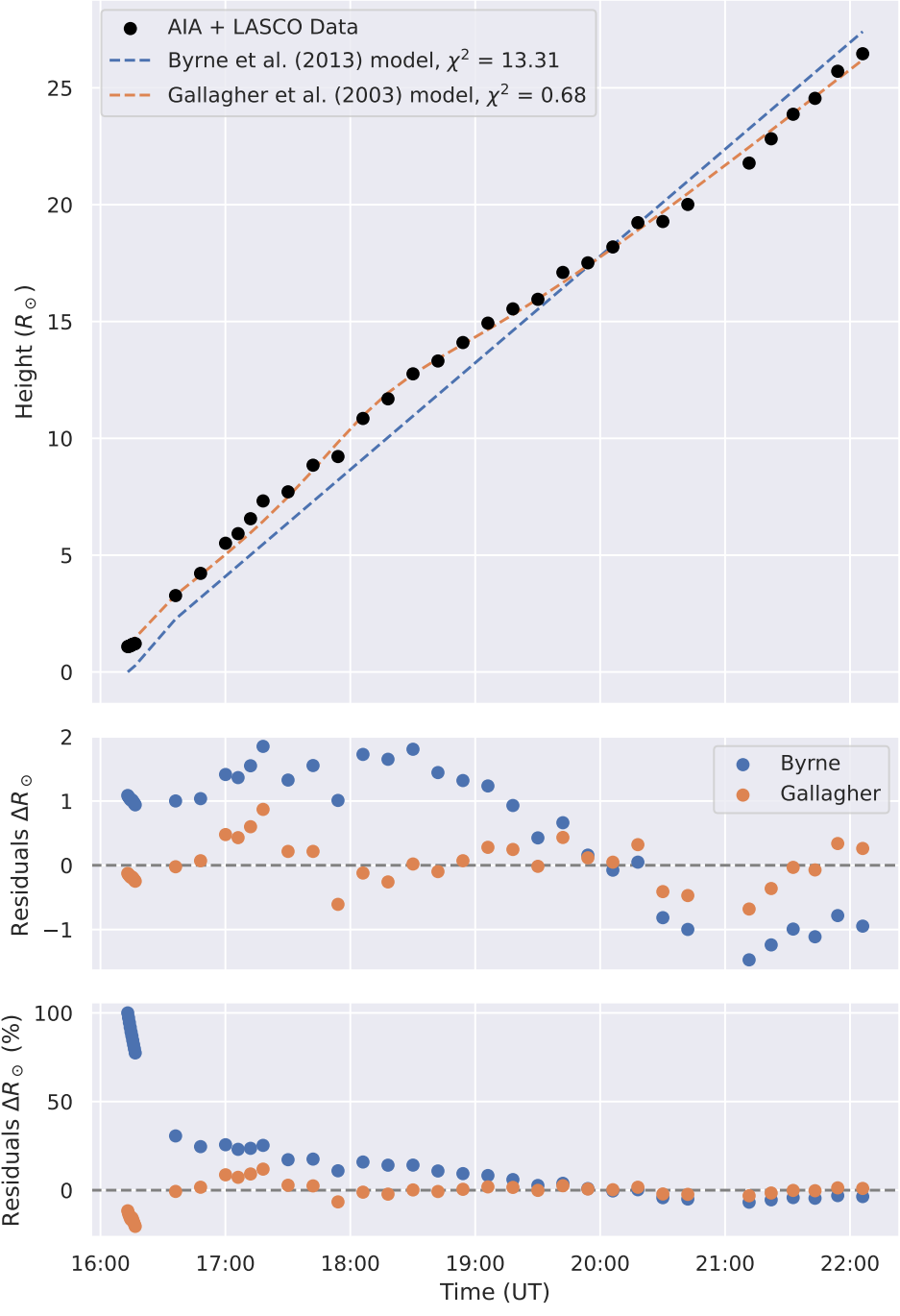
Figure A.19: Same for the event on July 8, 2014.
