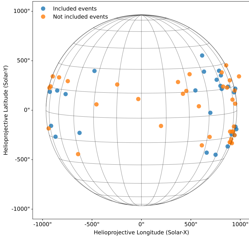
Figure 2.1: Distribution of the source location of the CBFs on the solar disk. The blue dots are the events that we included in Table 2.1, while the orange dots are the events that we did not include in the table.
