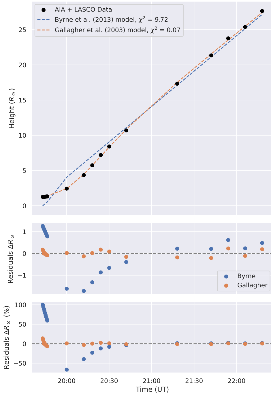
Figure A.5: Same for the event on March 7, 2011.
