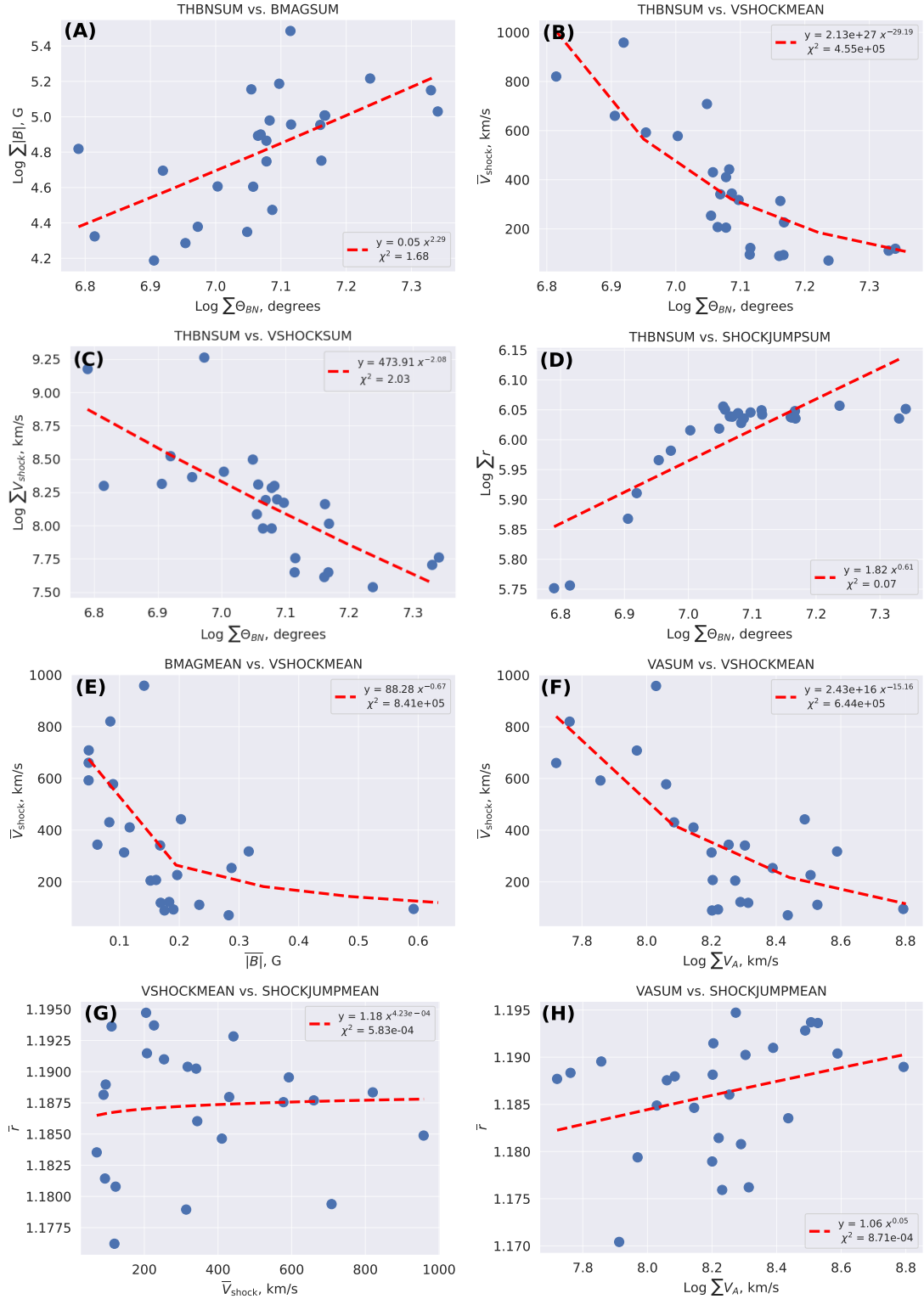
Figure 2.11: Scatter plots of 8 coronal plasma-parameter pairs that exhibit parameterizable relationships. The VSHOCKMEAN is filtered to take only events with speeds < 4000 \text{ km s}^{-1} .
