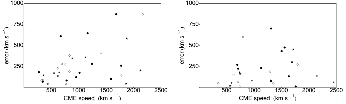
Figure 2.19: Scatter plot illustrates the comparison of 3D de-projected CME speeds derived from the spheroid model (depicted as diamonds), the ellipsoid model (represented by stars), and the GCS model (indicated as dots) versus the measurement errors for observers 1 (left) and 2 (right). Credit goes to Miteva et al. (2023).
