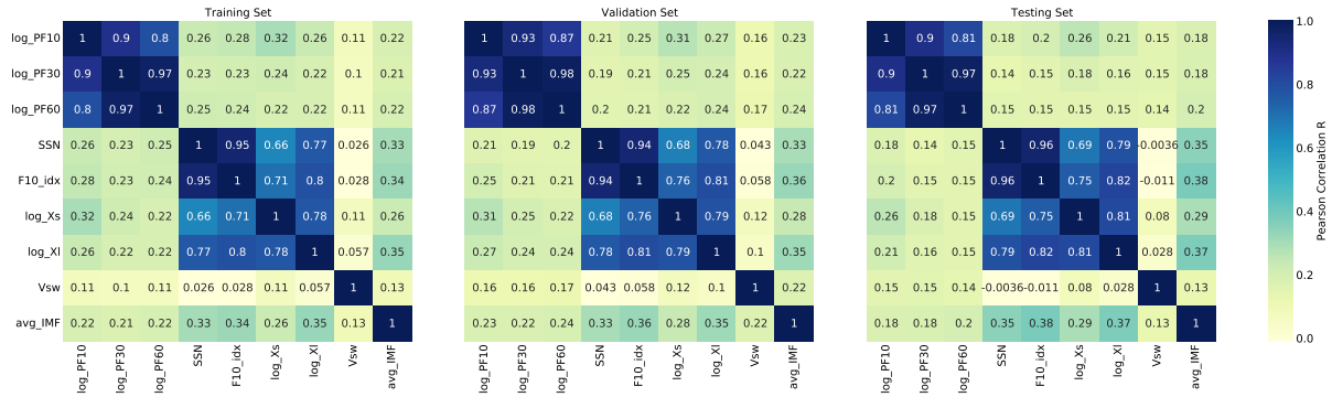
Figure 4.2: Correlation matrices show the correlation between the features in the training, validation, and test sets.
