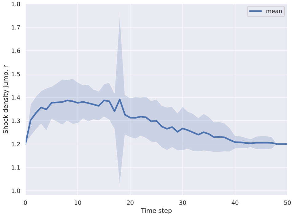
Figure 2.12: Time profile of the mean shock density jump for the 26 in-sample historical events studied with SPREADFAST.
