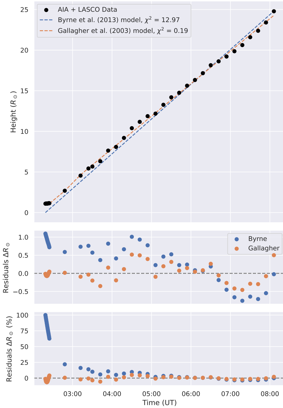
Figure A.21: Same for the event on May 12, 2015.
