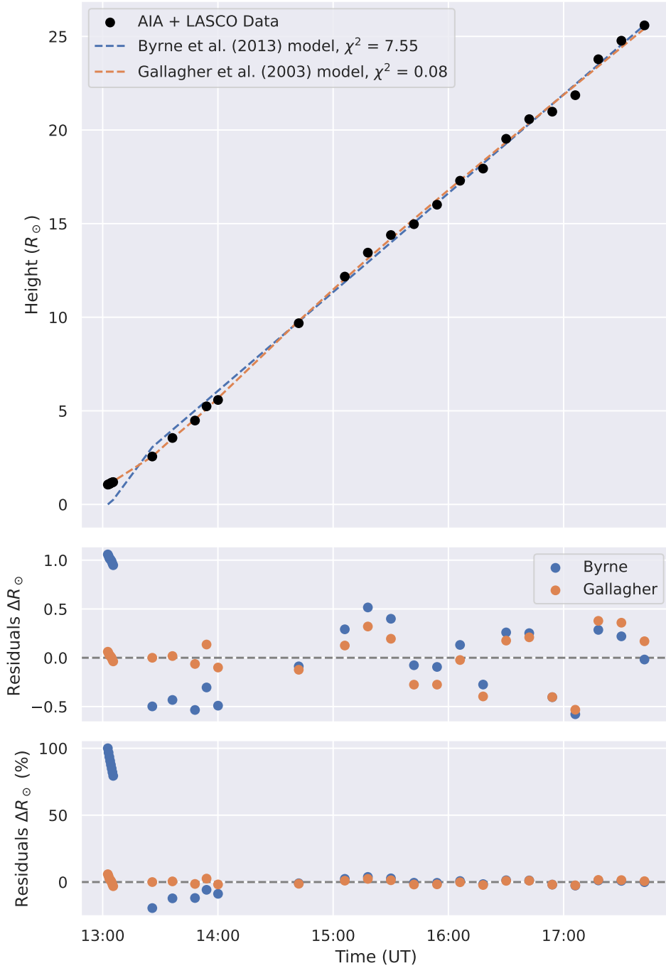
Figure A.24: Same for the event on November 9, 2015.
