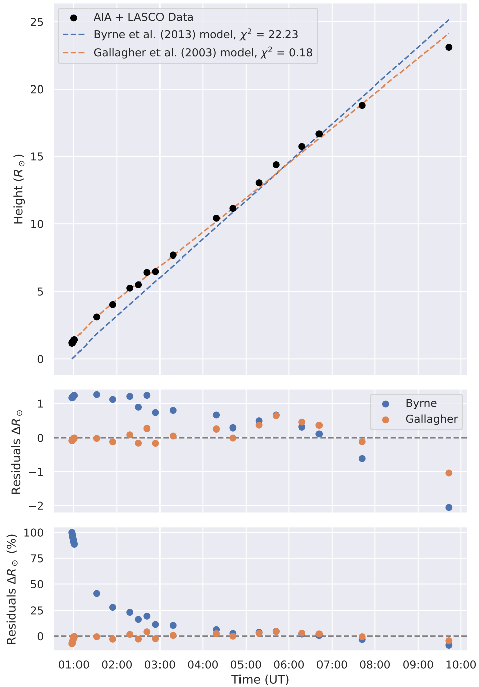
Figure A.1: Top panel: Height-time profile on June 12, 2010, using AIA and LASCO data, fitted with two CME kinematics models. Middle panel: Fitting vs. real observation difference. Bottom panel: Relative residuals in %.
