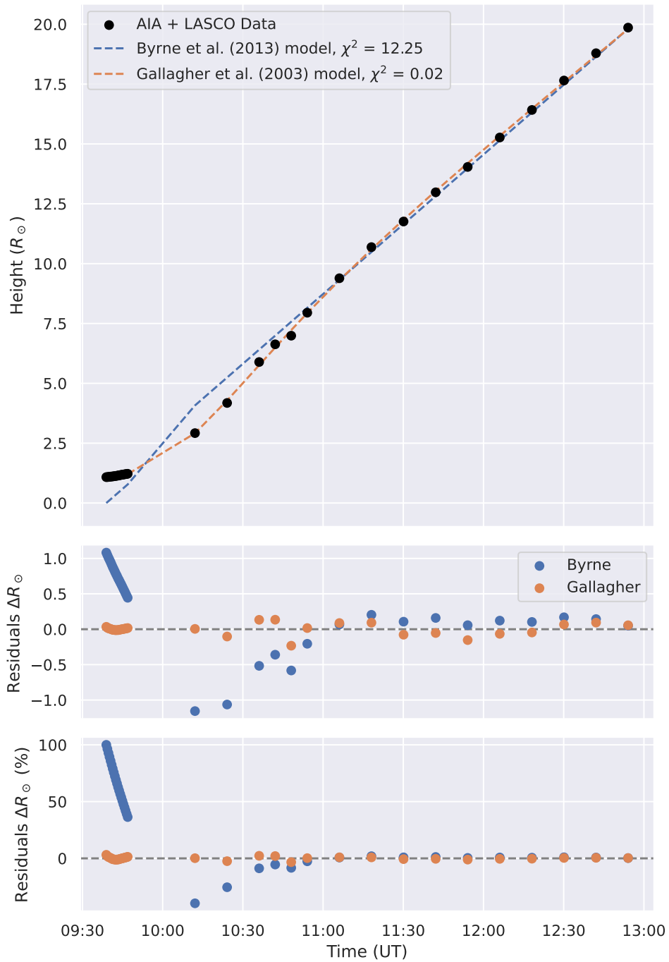
Figure A.2: Same for the event on August 14, 2010.
