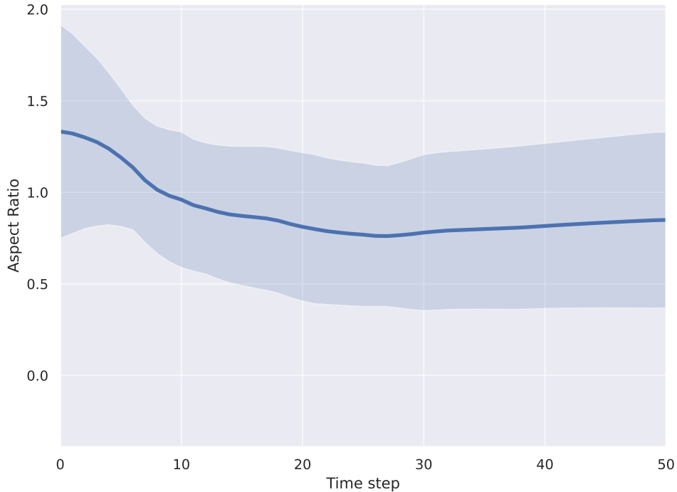
Figure 2.13: Time profile of the mean aspect ratio of the 26 historical events studied with SPREAdFAST.
