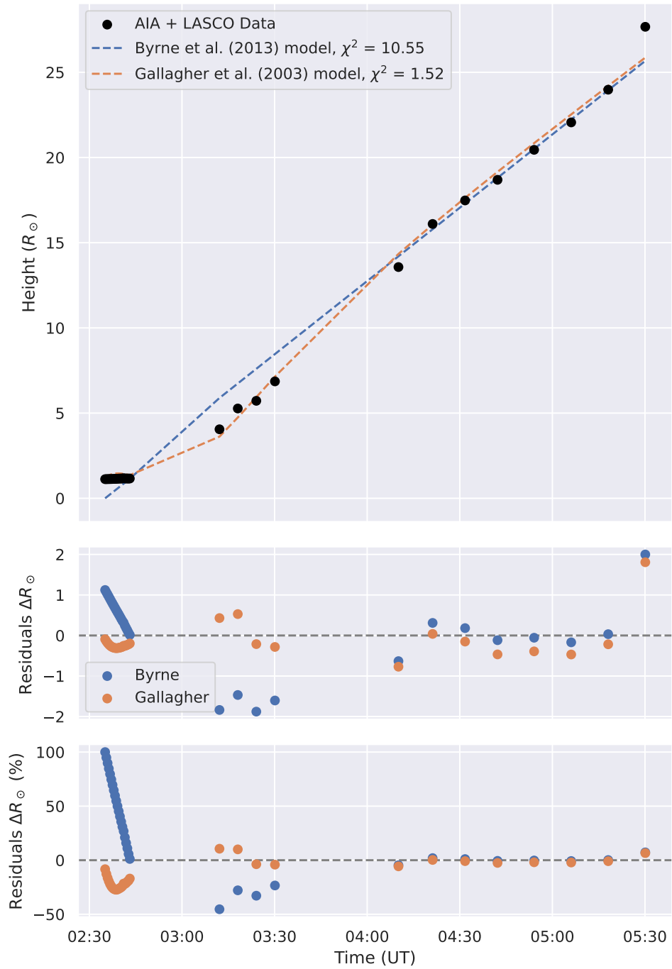
Figure A.15: Same for the event on June 21, 2013.
