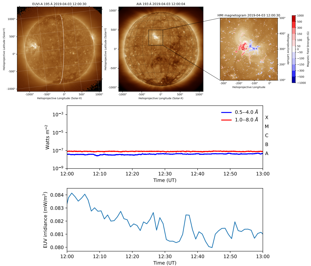
Figure 3.3: Exploring the X-ray and extreme ultraviolet (EUV) emissions from the Sun. The top panel showcases a cutout region of the SDO/AIA 193 Å image of the solar disk along with the STEREO-A EUVI 195 Å point of view. The white curve is the limb of the solar disk as seen by AIA from the right side. The red and blue colors are the contours of the line-of-sight magnetogram from the SDO/HMI instrument. The levels are (50, 100, 150, 300, 500, 1000) Gauss. The middle panel shows the X-ray flux from the GOES-14 spacecraft shows minimum activity. The bottom panel shows the time series of the ESP Quad band from the SDO/EVE instrument, which shows the solar irradiance in the extreme ultraviolet (EUV) band.
