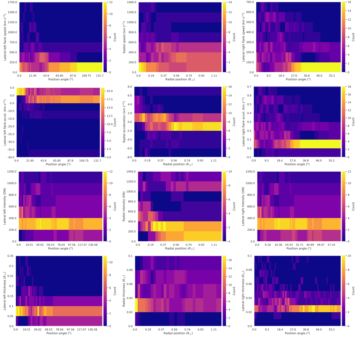
Figure 2.9: Dynamic spectra of the EUV waves kinematics in the AIA FOV. The panels from the top to the bottom are the wave speeds, acceleration, mean intensity, and thickness. The left column is for the lateral left flank, the central column is for the radial direction, and the right column is for the lateral right flank.
