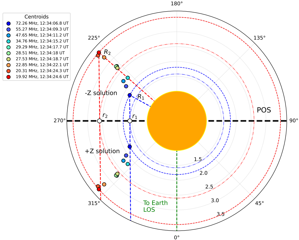
Figure A.26: Schematic shows the locations of the radio sources for the +Z and -Z solutions of Equation 3.4. The Sun is located in the middle as an orange circle, with a horizontal dashed black line representing the POS. The vertical dashed green line represents the Sun-Earth LOS. The dashed blue and red circles represent the plasma spheres of density equivalent to the observation frequencies of the innermost and outermost radio sources at R_1 and R_2 , respectively, under the Newkirk model assumption of spherically-symmetric density distribution. The impact parameters r_1 and r_2 are the projection of R_1 and R_2 on the POS. The dot-dashed blue and red circles are the circles passing through the impact parameters r_1 and r_2 , respectively.
