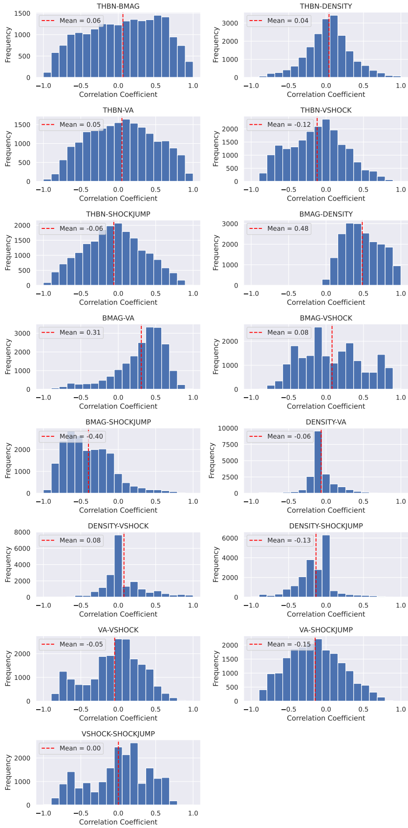
Figure 2.10: Histograms of along-field-lines model plasma parameters in the solar corona for all the 26 events. The vertical dashed red lines are the mean values.
