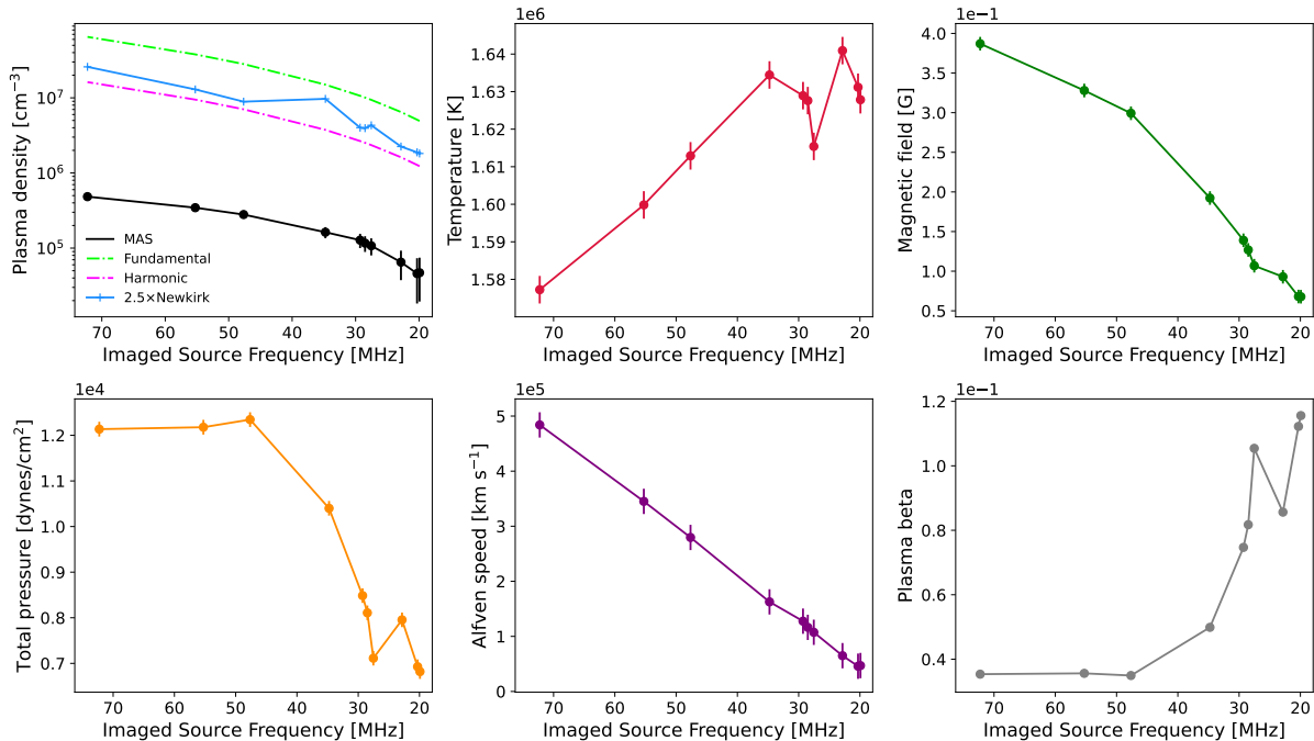
Figure 3.9: Coronal plasma parameters sampled from the 2D maps by the source centroids. The top panel shows (from left to right) the plasma density profiles from the MAS model, 2.5×Newkirk model, and the theoretical densities under the fundamental and harmonic assumptions, plasma temperature, and magnetic field. The bottom panel shows, from left to right, the total plasma dynamic pressure, Alfvén speed, and plasma beta. The x-axis is inverted to demonstrate a progression of increasing radial distance from the Sun as the observer moves towards the right.
