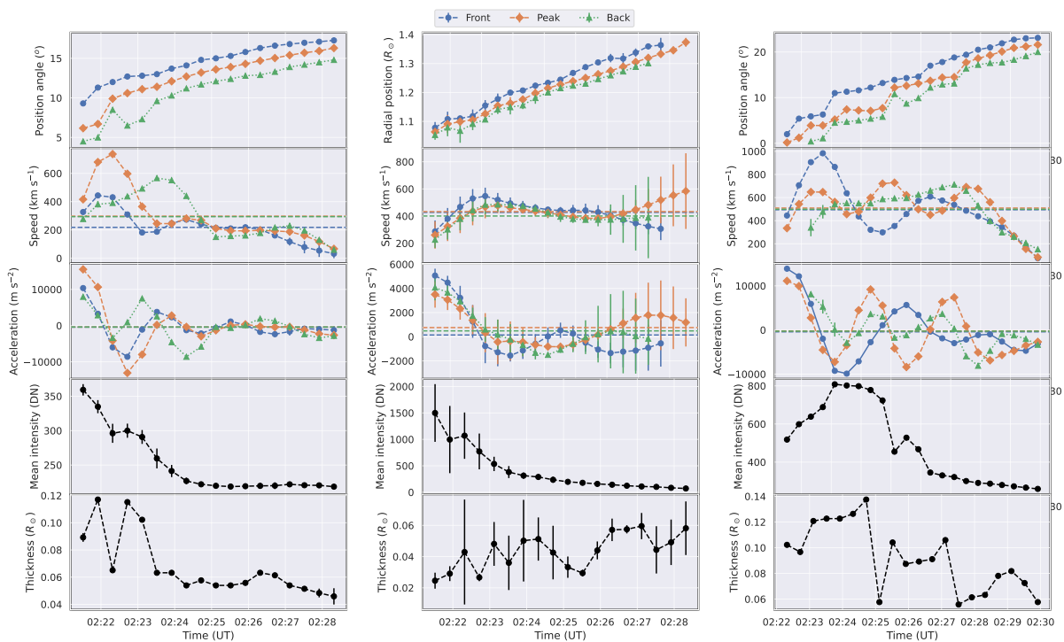
Figure 2.6: Time-series kinematics of the CBF parameters for the front, peak, and back positions in the AIA FOV, with measurement uncertainties shown as small bars over the data points. The horizontal lines in the speed and acceleration panels denote the mean speeds and accelerations for the wave front, peak, and back with respective colors. The left and right columns represent the lateral kinematic measurements in the left and right flanks of the wave, respectively. The middle column represent the kinematic measurements in the radial direction.
