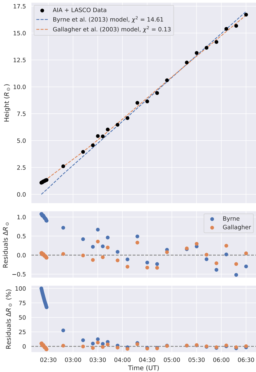
Figure 2.7: Top panel – Height-time profile compiled from AIA and LASCO measurements for the event occurred on May 11, 2011, fitted with two CME kinematics models from the photosphere up to 17 R_{\odot} . Middle panel – Difference between the fitting and the real observations. Bottom panel – Relative residuals in %.
